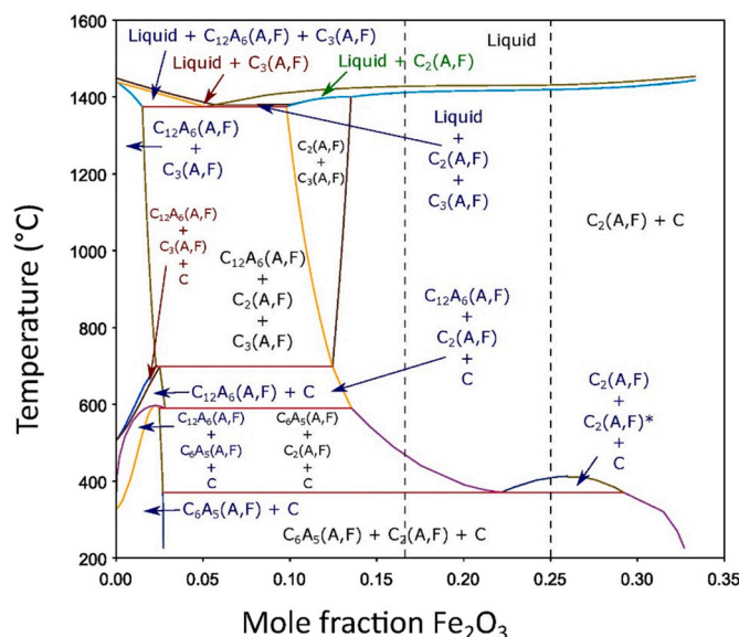
Fig. 7. Isopleth in the CaO- \text{Fe}_2\text{O}_3 - \text{Al}_2\text{O}_3 ternary diagram in air ( p(\text{O}_2) = 0.21 atm) where x(\text{CaO}) = 0.6667 showing ferrite \text{C}_2(\text{A},\text{F}) stability calculated using Thermo-Calc 2020b software and OXDEMO: Oxide demo database v2.0.
