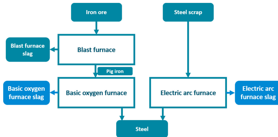
Fig. 1. Block-flow diagram of primary and secondary steel production.
